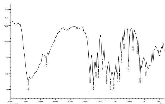
Gambar 6. Spektrum FTIR standar kuersetin
